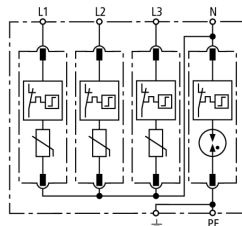
Basic circuit diagram DG M TT 150
