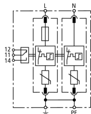
Basic circuit diagram DG M TN CI 275 FM
