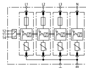
Basic circuit diagram DG M TNS CI 275
